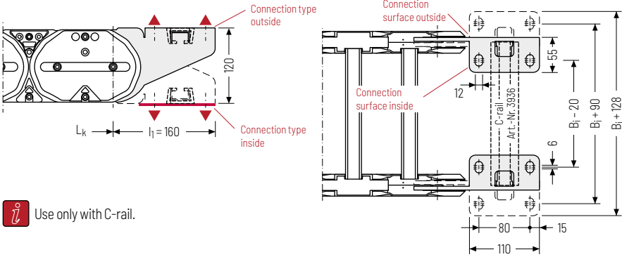
▲ Assembly options
